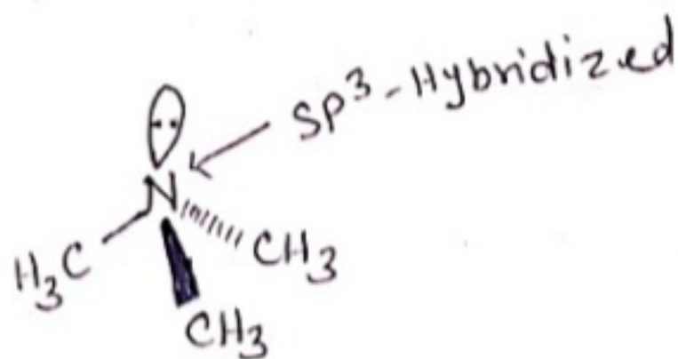
Trimethylamine ( 3^\circ )
