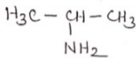
Isopropylamine
