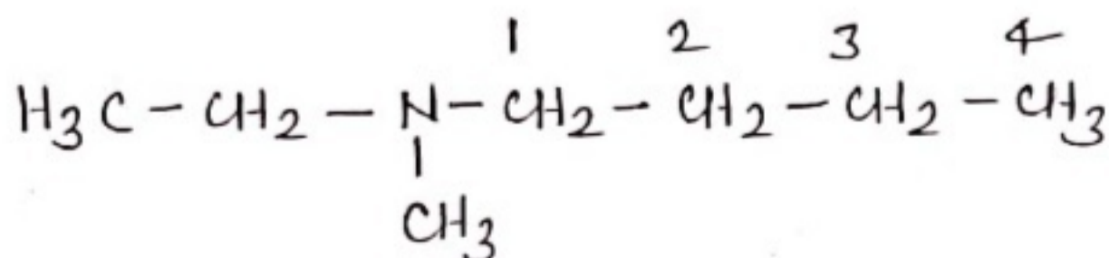
N-ethyl-N-methylbutan-1-amine.
