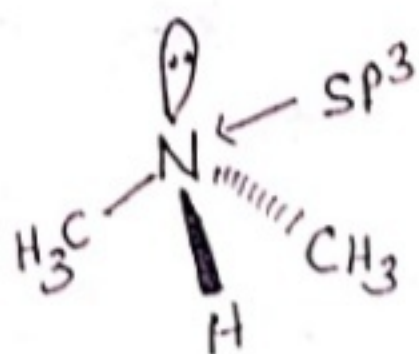
Dimethylamine ( 2^\circ )
