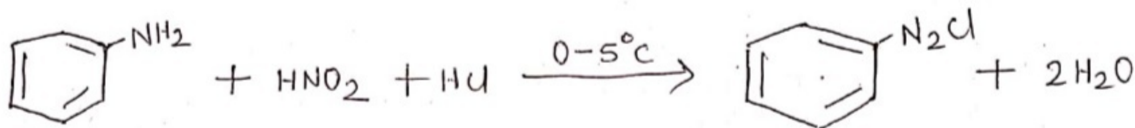
Benzene diazonium chloride
