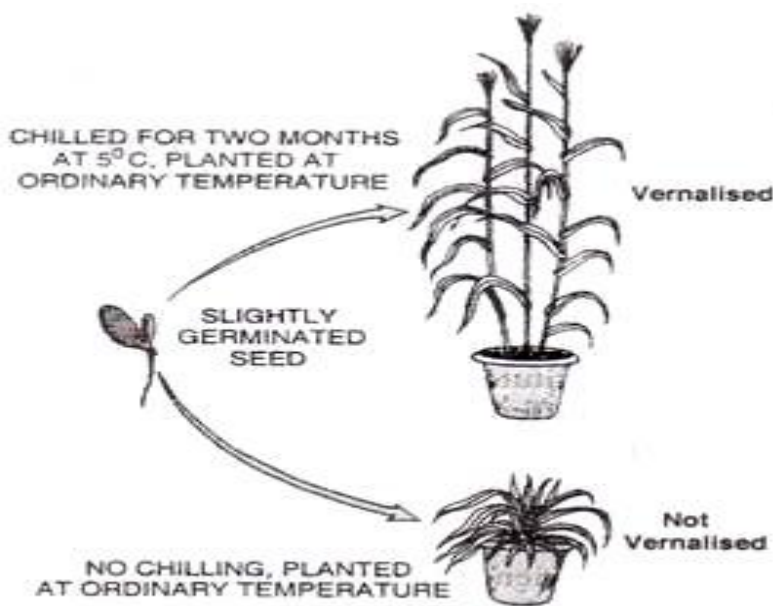
Fig. 15.33. Experiment to show effect of vernalization on Winter Rye.
