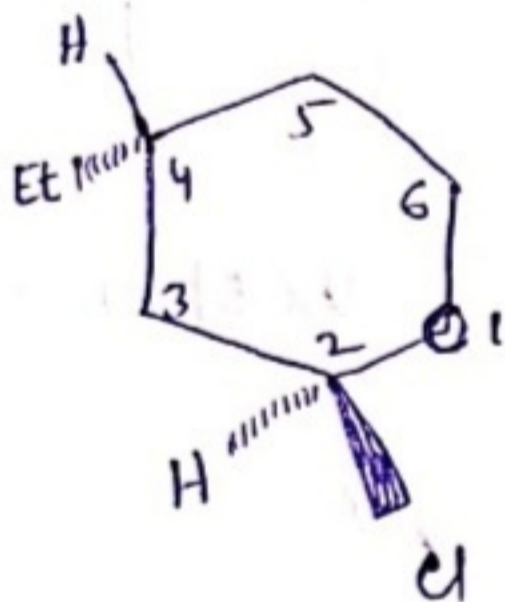
trans 2-chloro-4-ethyloxane
