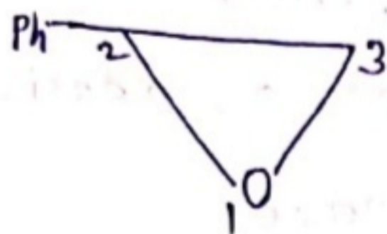
2-phenyloxirane
