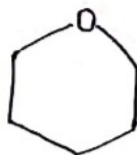
Oxane
