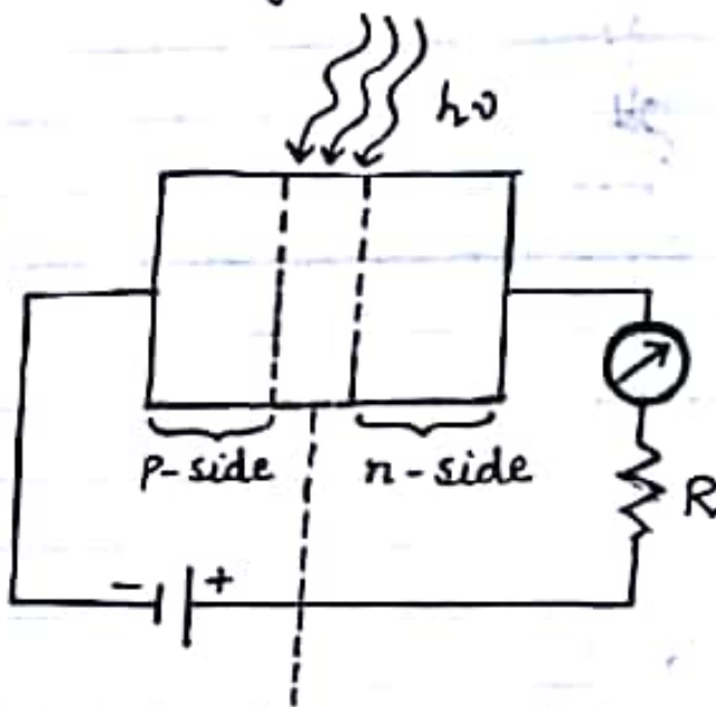
Fig. 2 :- A reverse biased photodiode illuminated with light.
