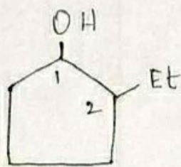
2-ethylcyclopentan-1-ol
