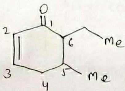
6-ethyl-5-methylcyclohex-2-en-1-one
