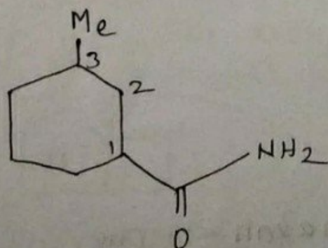
3-methylcyclohexane-1-carboxamide
