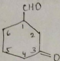
3-oxocyclohexane carbaldehyde
