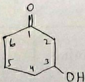
3-Hydroxycyclohexan-1-one
