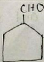
cyclopentane carbaldehyde
