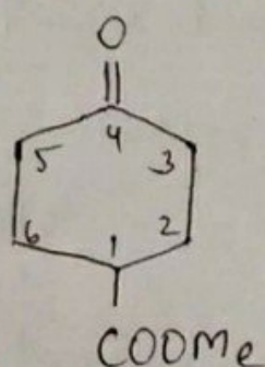
methyl (4-oxocyclohexane)-1-carboxylate
