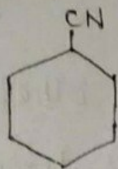
cyclohexane carbonitrile
